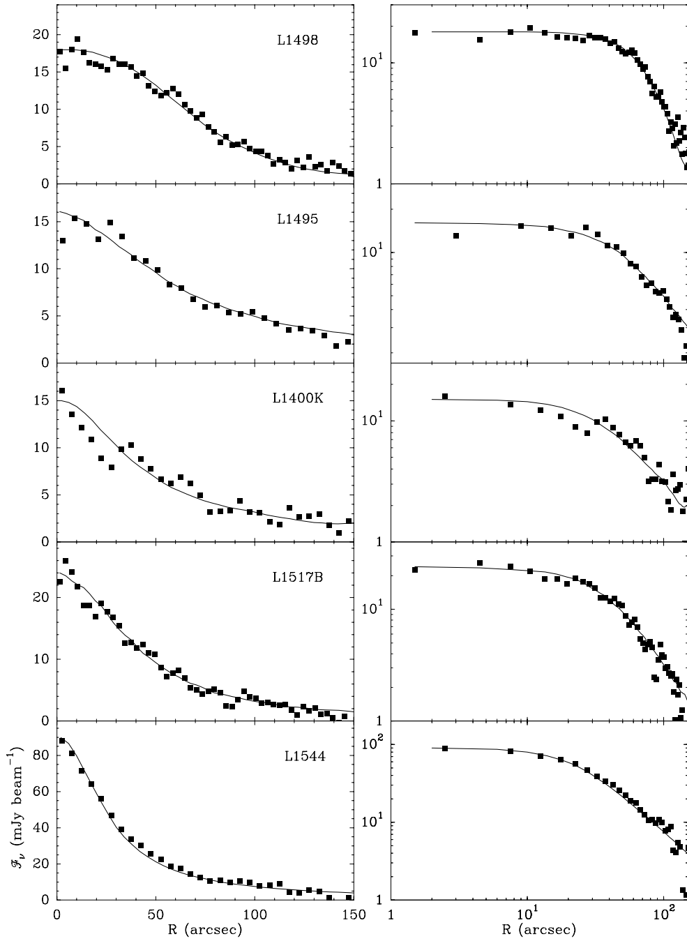
FIG. 2.— Radial profiles of 1.2mm continuum emission in both linear and log-log scale. (L1544 data from Ward-Thompson et al. 1999.) Solid squares are telescope measurements and lines are models for which a simulation of an on-the-fly observation has been done (see text). For L1495 and L1517B, the profiles represent circular averages, while for L1498, L1400K, and L1544, they represent elliptical averages with the parameters shown in Table 2. See also Table 2 for the input parameters of the models. Scale is in mJy/11''-beam for L1498, L1495, L1400K, and L1517B, and mJy/13''-beam for L1544. In contrast to Fig. 1, the data from the first four cores have not been convolved additionally after the telescope observation.
